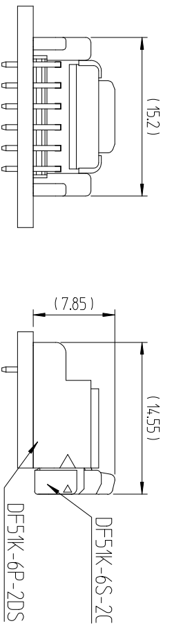
ENGAGEMENT FIGURE (2:1)
