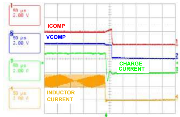
FIGURE 8. CHARGE DISABLE
