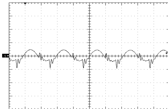
Figure 8. . Output Voltage Ripple (20mV/div), time scale – 1uS/div. Vin=Vin_nom, full load Cout=0.1uF ceramic + 10uF Tantalum (see Fig 16)
