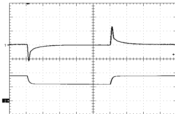
Figure 12. Load Transient Response (50mV/div), di/dt=0.1A/uS, 50%-75%-50% of full load, Cout=Fig16 time scale: 200uS/div. Ch1=Vout, Ch2=Iout (1A/div)
