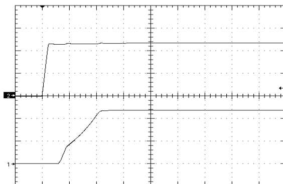
Figure 10. Startup Waveform via Input Voltage, time scale 10mS/div. Vin=Vin_nom, Iout=full load Cout=2000uF, Ch1=Vout (5V/div), Ch2=Vin (10V/div)
