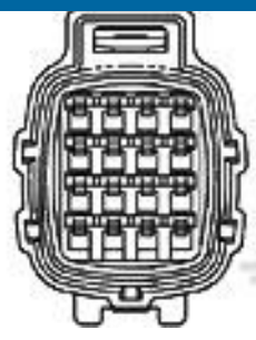
TE Part #368047-1 E-S MK-2(+) 16P PLUG ASSY
