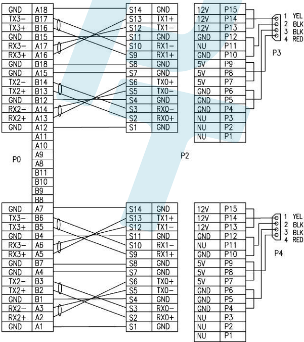
WIRING DIAGRAM
