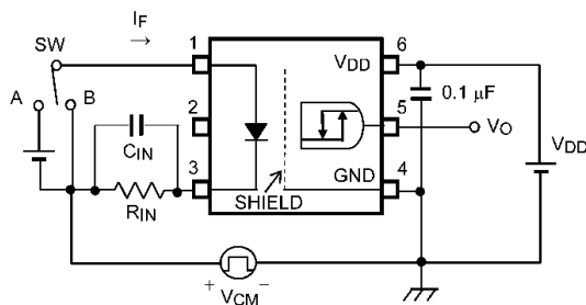
Fig. 12.1.5 Switching Time Test Circuit and Waveform
