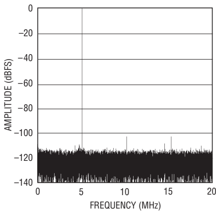
LTC2204: 64K Point FFT, 40Msps, f_{IN} = 5.1\text{MHz} , -1\text{dBFS} , \text{PGA} = 1 , \text{DITH} = 0
