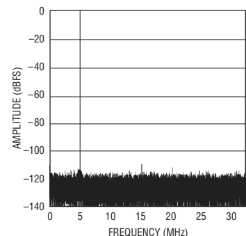
LTC2205: 64K Point FFT, f_{IN} = 5.1\text{MHz} , -1dBFS, PGA = 0, DITH = 0
