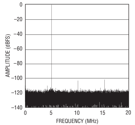
LTC2204: 64K Point FFT, 40Msps, f_{IN} = 5.1\text{MHz} , -1\text{dBFS} , \text{PGA} = 0 , \text{DITH} = 0
