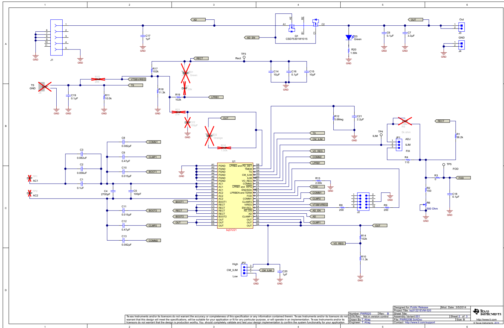
Figure 1. bq51221 EVM-520 Schematic
