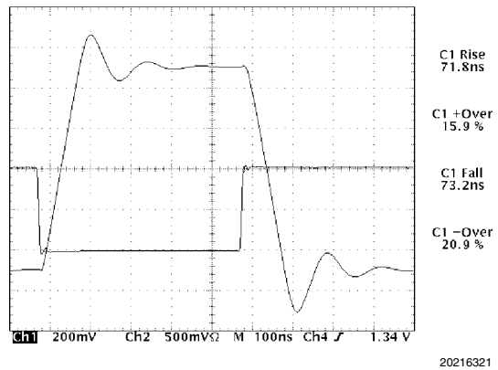
FIGURE 10. LMV796 Response
