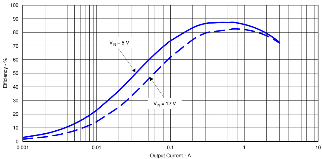
Figure 4-2. TPS54339EVM-056 Light-Load Efficiency
