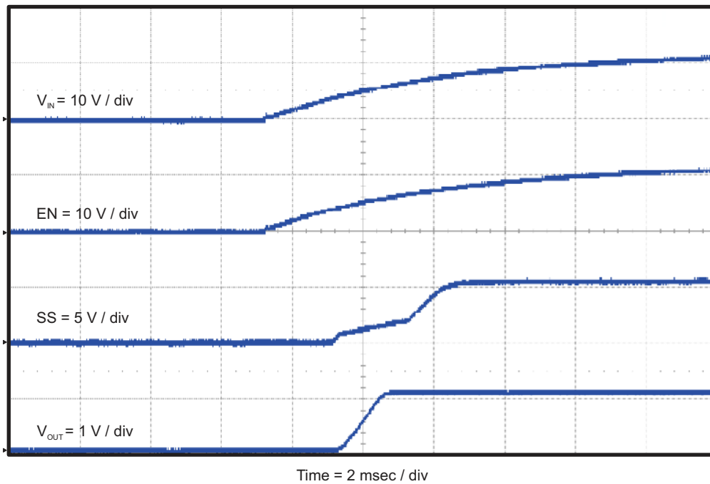
Figure 4-9. TPS54339EVM-056 Start-Up Relative to V_{IN} with SS
