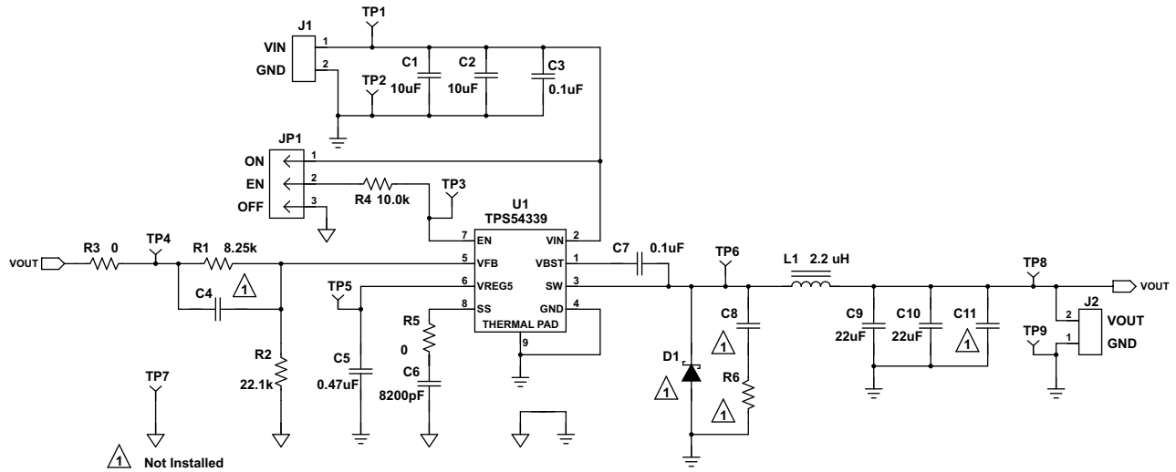
Figure 6-1. TPS54339EVM-056 Schematic Diagram
