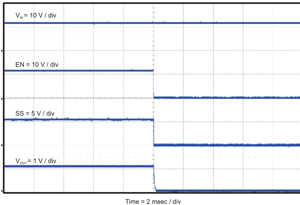
Figure 4-12. TPS54339EVM-056 Shut-Down Relative to EN with SS
