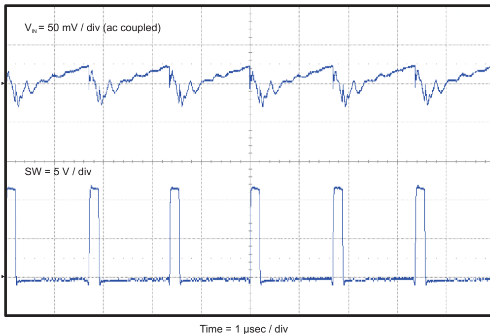
Figure 4-8. TPS54339EVM-056 Input Voltage Ripple
