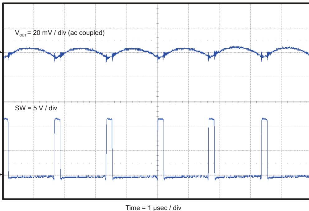
Figure 4-6. TPS54339EVM-056 Output Voltage Ripple ( I_{OUT} = 3 \text{ A} )
