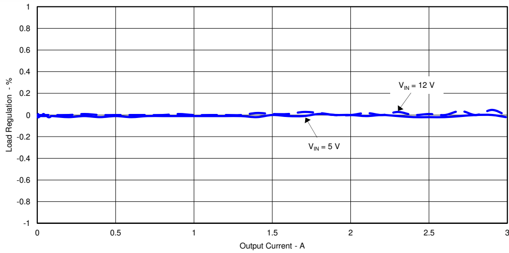
Figure 4-3. TPS54339EVM-056 Load Regulation, V_{IN} = 5\text{ V} and V_{IN} = 12\text{ V}
