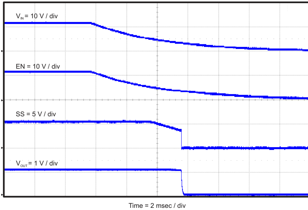
Figure 4-11. TPS54339EVM-056 Shut-Down Relative to V_{IN} with SS
