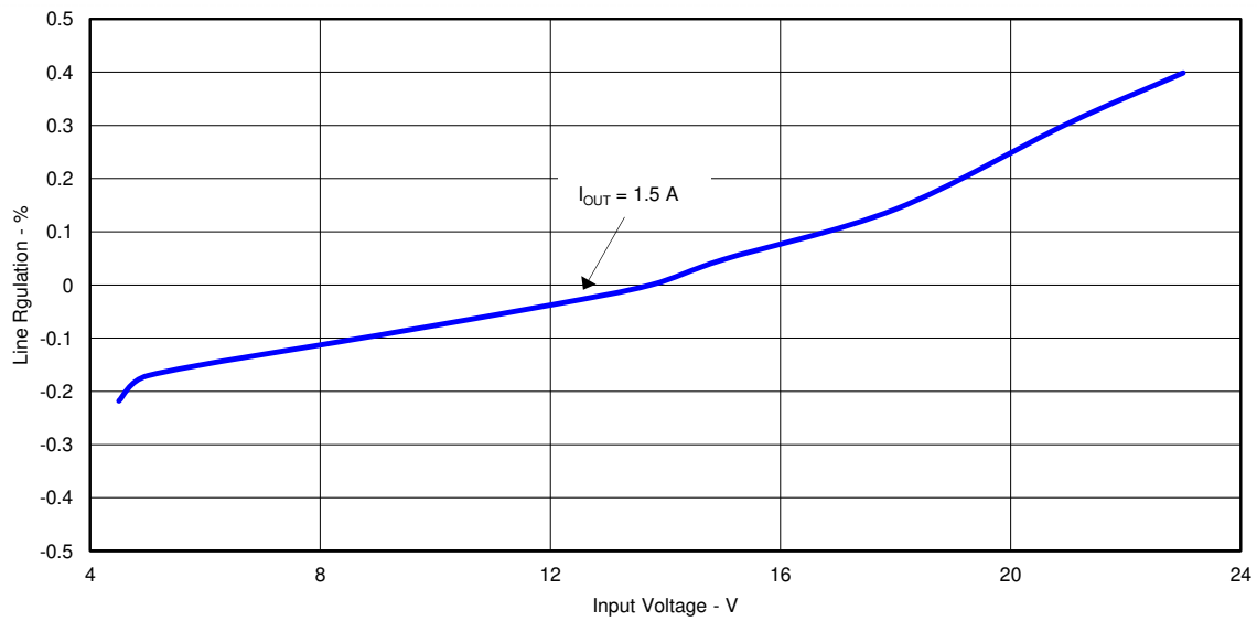
Figure 4-4. TPS54339EVM-056 Line Regulation
