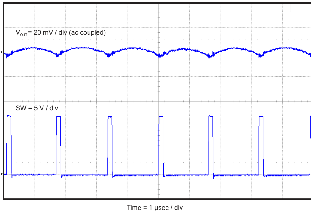
Figure 4-7. TPS54339EVM-056 Output Voltage Ripple ( I_{OUT} = 0 \text{ A} )
