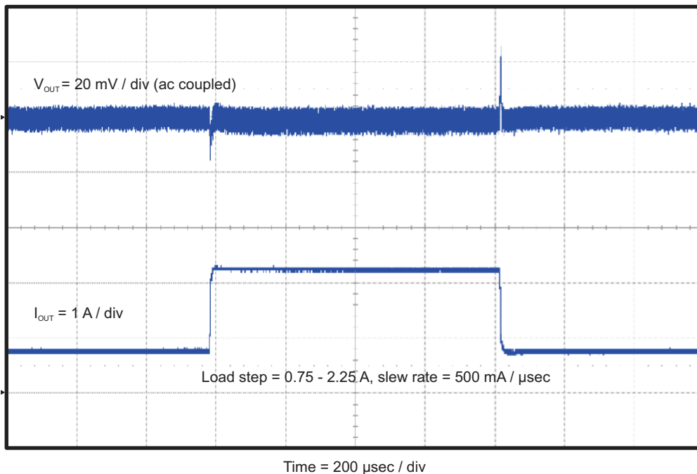
Figure 4-5. TPS54339EVM-056 Load Transient Response
