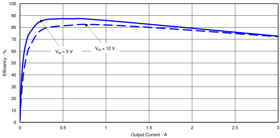
Figure 4-1. TPS54339EVM-056 Efficiency
