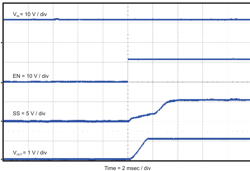
Figure 4-10. TPS54339EVM-056 Start-Up Relative to EN with SS
