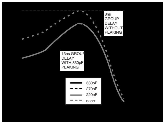
Figure 13. Group Delay at 5.5MHz (PAL) With and Without Peaking Capacitor
