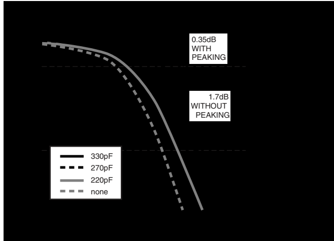
Figure 11. NTSC/PAL Video Frequency Response With and Without Peaking Capacitor
