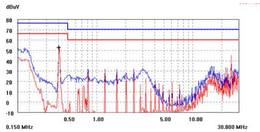
Figure 15. KNW015A0Fxx-88 Quasi Peak Conducted Emissions with EN 55022 Class A limits, Figure 14 filter ( V_{IN} = V_{IN,NOM} , I_o = 0.80 I_{o,max} ).
