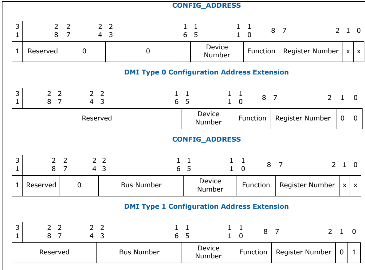
Figure 3. DMI Type 0 Configuration Address Translation
