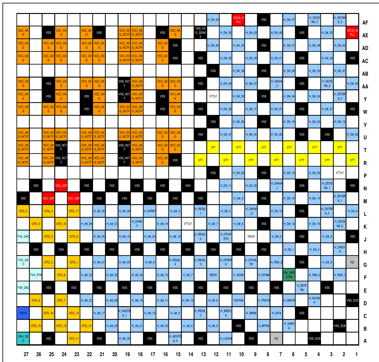
Figure 28. Ballout Diagram (Top View) Lower Right Quadrant
