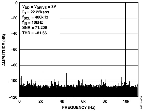
Figure 4. Typical FFT
