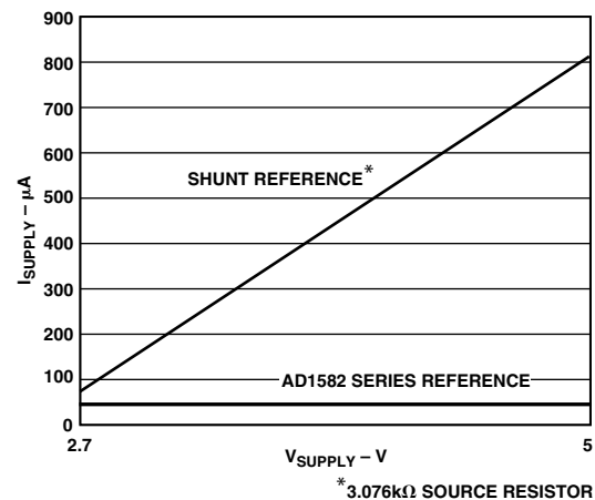
Figure 1. Supply Current ( \mu\text{A} ) vs. Supply Voltage (V)
