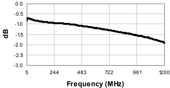
Amplitude Balance
