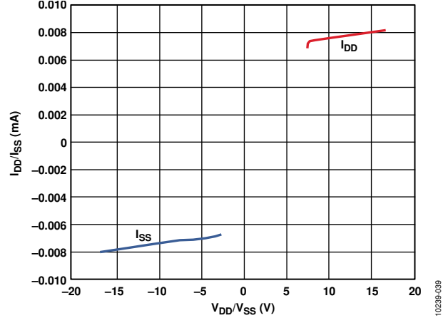
Figure 38. Power Supply Currents vs. Power Supply Voltages
