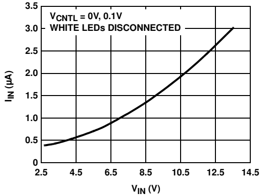
FIGURE 2. QUIESCENT CURRENT
