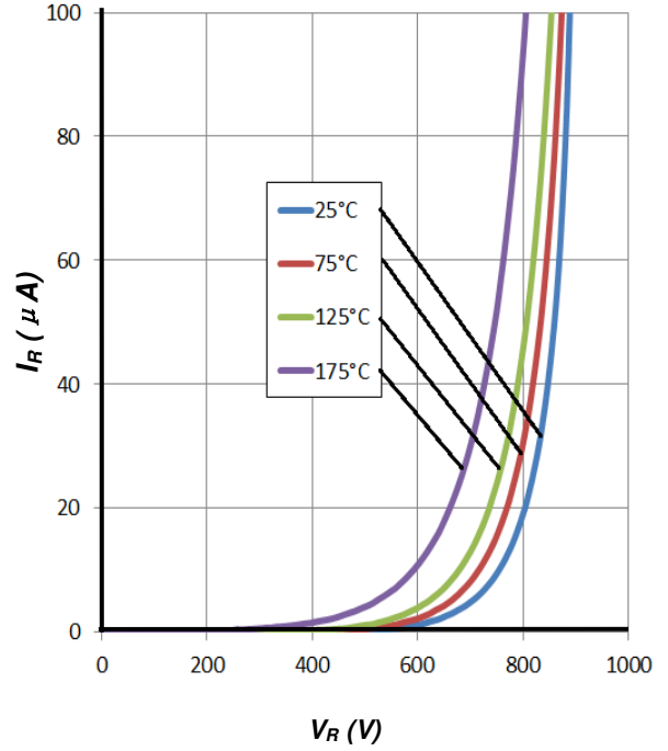
Figure 2. Reverse Characteristics
