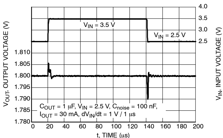
Figure 30. Line Transient Response, V OUT = 1.8 V, C OUT = 1 μF, I OUT = 30 mA
