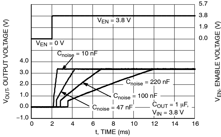
Figure 34. Turn-On Response V_{OUT} = 3.3 \text{ V} , C_{OUT} = 1 \mu\text{F} , I_{OUT} = 30 \text{ mA}
