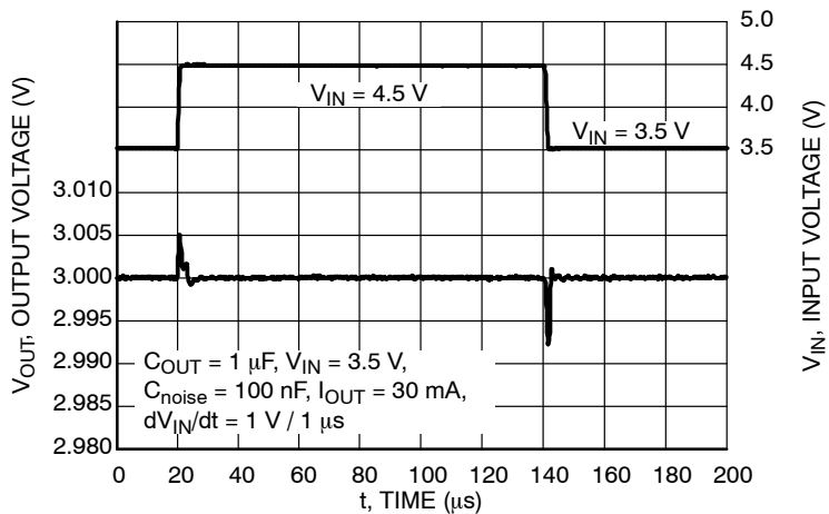
Figure 32. Line Transient Response, V OUT = 3.0 V, C OUT = 1 μF, I OUT = 30 mA
