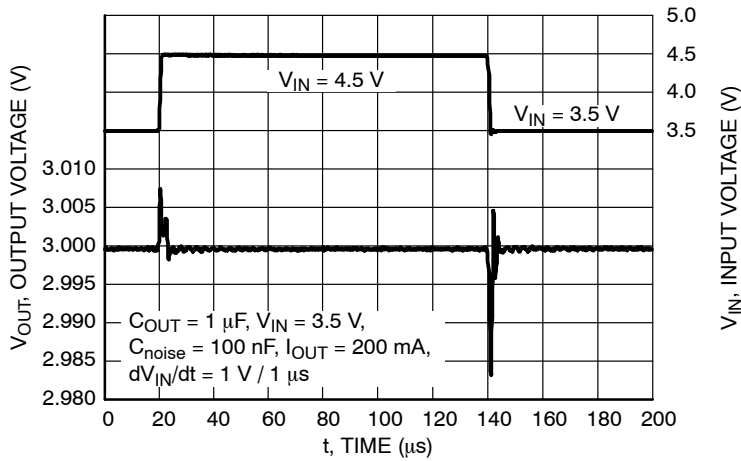
Figure 33. Line Transient Response, V_{OUT} = 3.0 \text{ V} , C_{OUT} = 1 \mu\text{F} , I_{OUT} = 200 \text{ mA}
