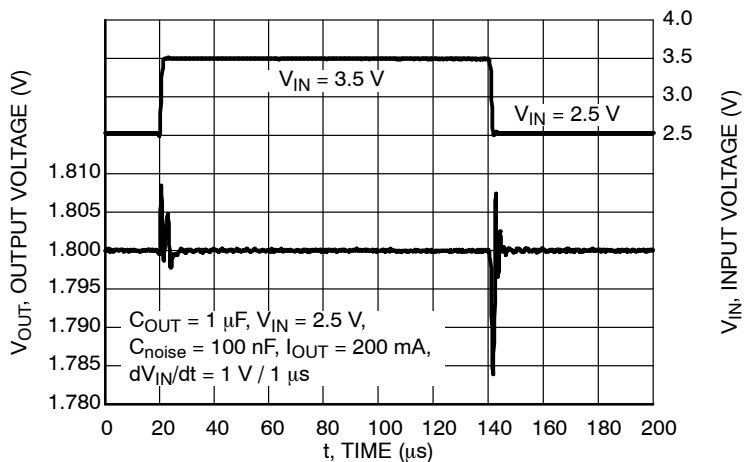
Figure 31. Line Transient Response, V OUT = 1.8 V, C OUT = 1 μF, I OUT = 200 mA
