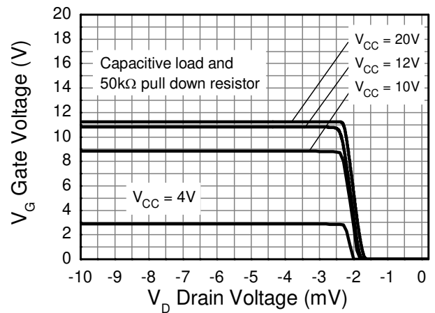
Transfer Characteristic
