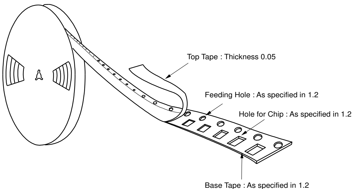
Fig3 Taping Diagram
