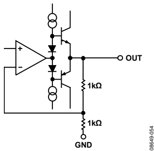
Figure 52. ADV3220 Enabled Analog Output
