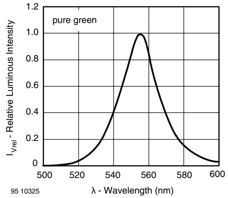
Figure 29. Relative Intensity vs. Wavelength
