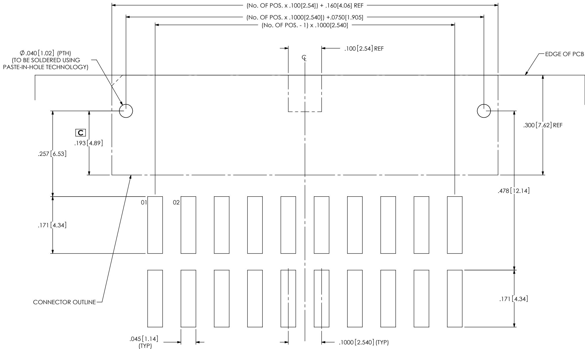
FIG. 1 (IPL1-110-01-XXX-DH-K SHOWN)
