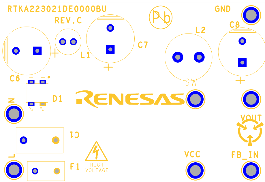
Figure 7. Top Layer
