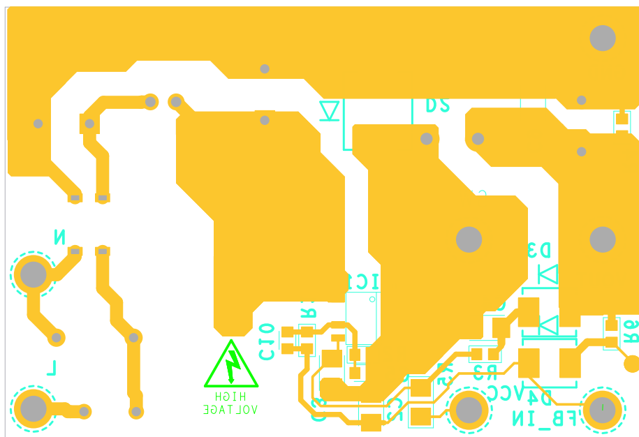
Figure 8. Bottom Layer
