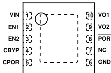
ISL9012 (10 LD 3X3 DFN) TOP VIEW
