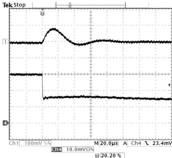
Fig-1.8V-6: Output voltage response for V_{out}=1.8V to positive load current step change from 1.5A to 3A with slew rate of 5A/\mu s at V_{in}=12V . C_o=47\mu F \times 2 ceramic.
