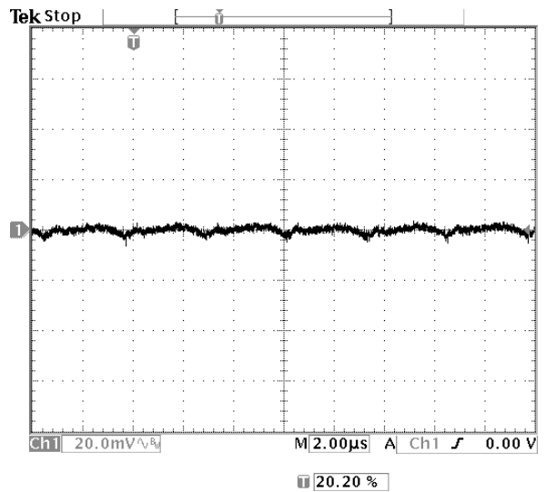
Fig-1.5V-5: Output voltage ripple (20mV/div.) for V_{out}=1.5V at full rated load current into a resistive load with external capacitance 47\mu F \times 2 ceramic + 1\mu F ceramic at V_{in}=12V .
