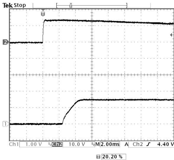
Fig-1.5V-4: Turn-on transient for V_{out}=1.5V with application of V_{in} at full rated load current (resistive) and 47\mu F \times 2 external capacitance at V_{in}=12V .
