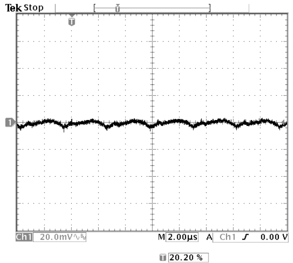
Fig-2.0V-5: Output voltage ripple (20mV/div.) for V_{out}=2.0V at full rated load current into a resistive load with external capacitance 47\mu F \times 2 ceramic + 1\mu F ceramic at V_{in}=12V .
