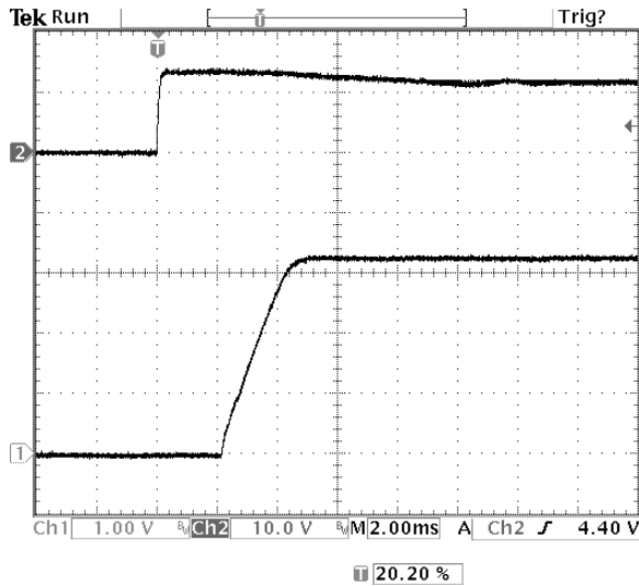
Fig-3.3V-4: Turn-on transient for V_{out}=3.3V with application of V_{in} at full rated load current (resistive) and 47\mu F \times 2 external capacitance at V_{in}=12V .
