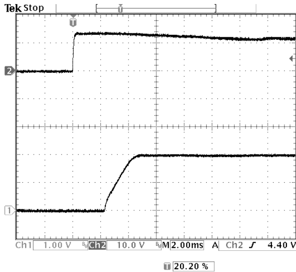
Fig-2.0V-4: Turn-on transient for V_{out}=2.0V with application of V_{in} at full rated load current (resistive) and 47\mu F \times 2 external capacitance at V_{in}=12V .
