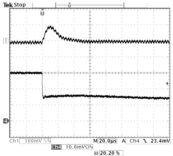
Fig-5.0V-7: Output voltage response for V_{out}=5.0V to negative load current step change from 3A to 1.5A with slew rate of -5A/\mu s at V_{in}=12V . C_o=47\mu F \times 2 ceramic.
