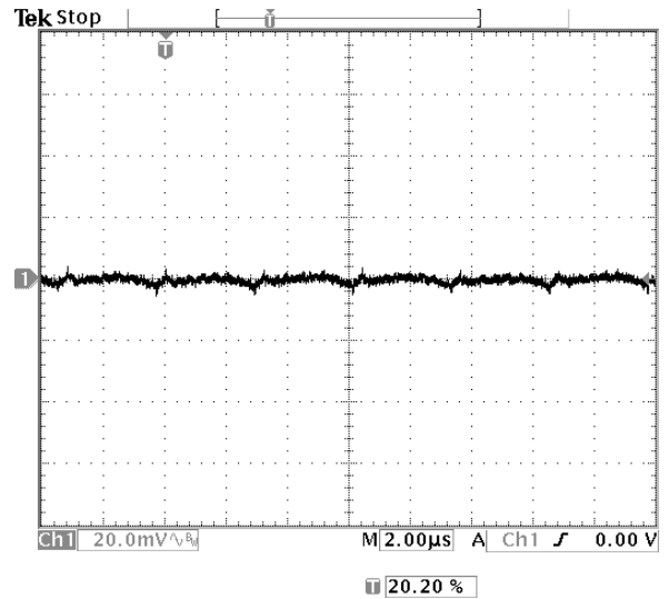
Fig-1.0V-5: Output voltage ripple (20mV/div.) for V_{out}=1.0V at full rated load current into a resistive load with external capacitance 47\mu F \times 2 ceramic + 1\mu F ceramic at V_{in}=12V .
