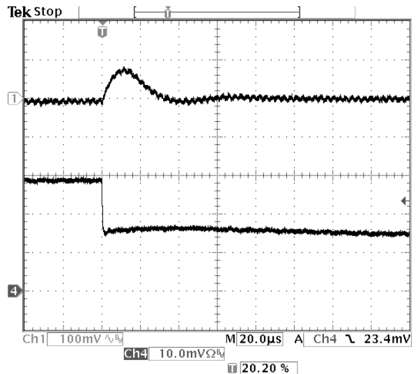
Fig-3.3V-7: Output voltage response for V_{out}=3.3V to negative load current step change from 3A to 1.5A with slew rate of -5A/\mu s at V_{in}=12V . C_o=47\mu F \times 2 ceramic.
