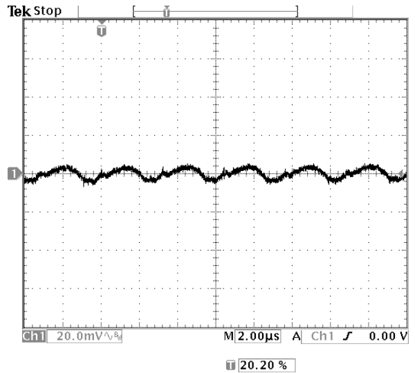
Fig-3.3V-5: Output voltage ripple (20mV/div.) for V_{out}=3.3V at full rated load current into a resistive load with external capacitance 47\mu F \times 2 ceramic + 1\mu F ceramic at V_{in}=12V .
