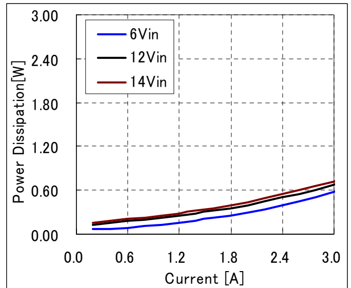
Fig-1.0V-3: Power dissipation vs. load current and input voltage for Vout=1.0V. Airflow rate=200 LFM (1m/s) and Ta=25°C.
