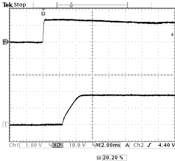
Fig-1.8V-4: Turn-on transient for V_{out}=1.8V with application of V_{in} at full rated load current (resistive) and 47\mu F \times 2 external capacitance at V_{in}=12V .
