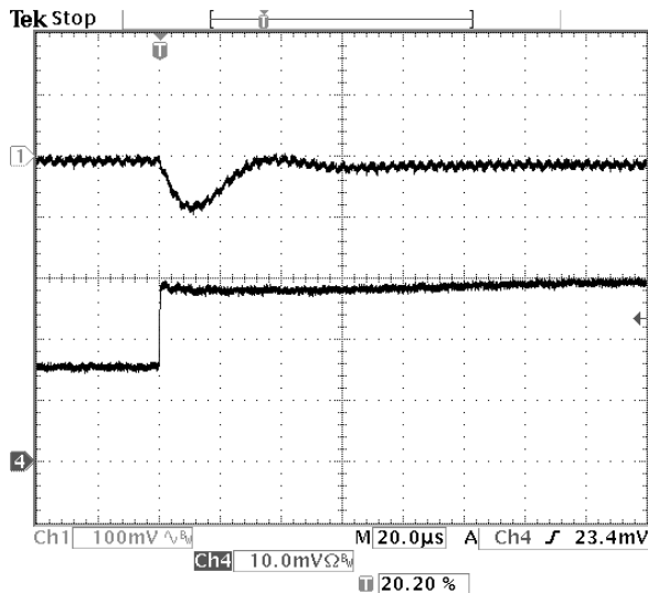
Fig-3.3V-6: Output voltage response for V_{out}=3.3V to positive load current step change from 1.5A to 3A with slew rate of 5A/\mu s at V_{in}=12V . C_o=47\mu F \times 2 ceramic.
