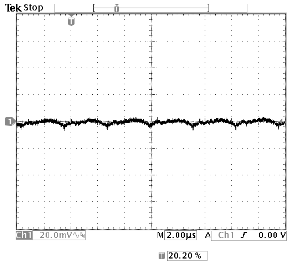
Fig-1.8V-5: Output voltage ripple (20mV/div.) for V_{out}=1.8V at full rated load current into a resistive load with external capacitance 47\mu F \times 2 ceramic + 1\mu F ceramic at V_{in}=12V .
