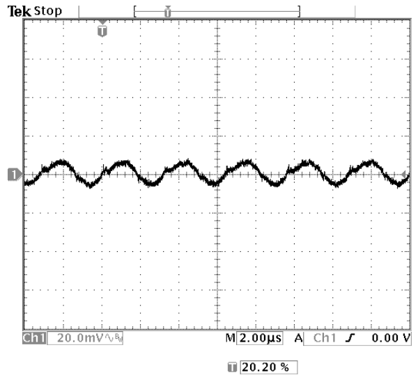
Fig-5.0V-5: Output voltage ripple (20mV/div.) for V_{out}=5.0V at full rated load current into a resistive load with external capacitance 47\mu F \times 2 ceramic + 1\mu F ceramic at V_{in}=12V .
