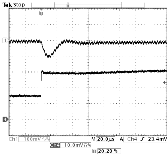
Fig-5.0V-6: Output voltage response for V_{out}=5.0V to positive load current step change from 1.5A to 3A with slew rate of 5A/\mu s at V_{in}=12V . C_o=47\mu F \times 2 ceramic.
