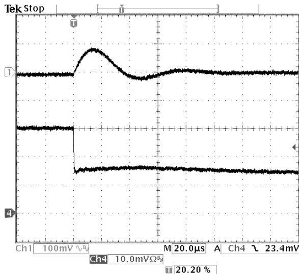
Fig-1.0V-6: Output voltage response for V_{out}=1.0V to positive load current step change from 1.5A to 3A with slew rate of 5A/\mu s at V_{in}=12V . C_o=47\mu F \times 2 ceramic.
