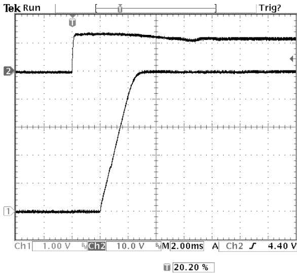
Fig-5.0V-4: Turn-on transient for V_{out}=5.0V with application of V_{in} at full rated load current (resistive) and 47\mu F \times 2 external capacitance at V_{in}=12V .
