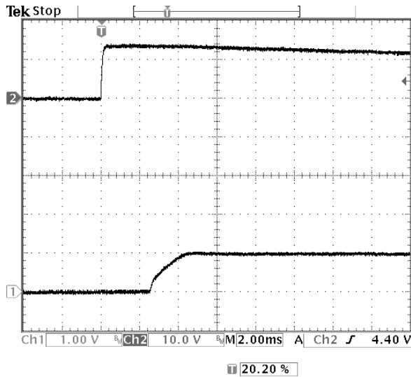
Fig-1.0V-4: Turn-on transient for V_{out}=1.0V with application of V_{in} at full rated load current (resistive) and 47\mu F \times 2 external capacitance at V_{in}=12V .
