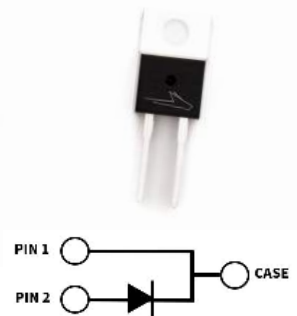
Package Types: TO-220-2 Marking: C3D06060A
