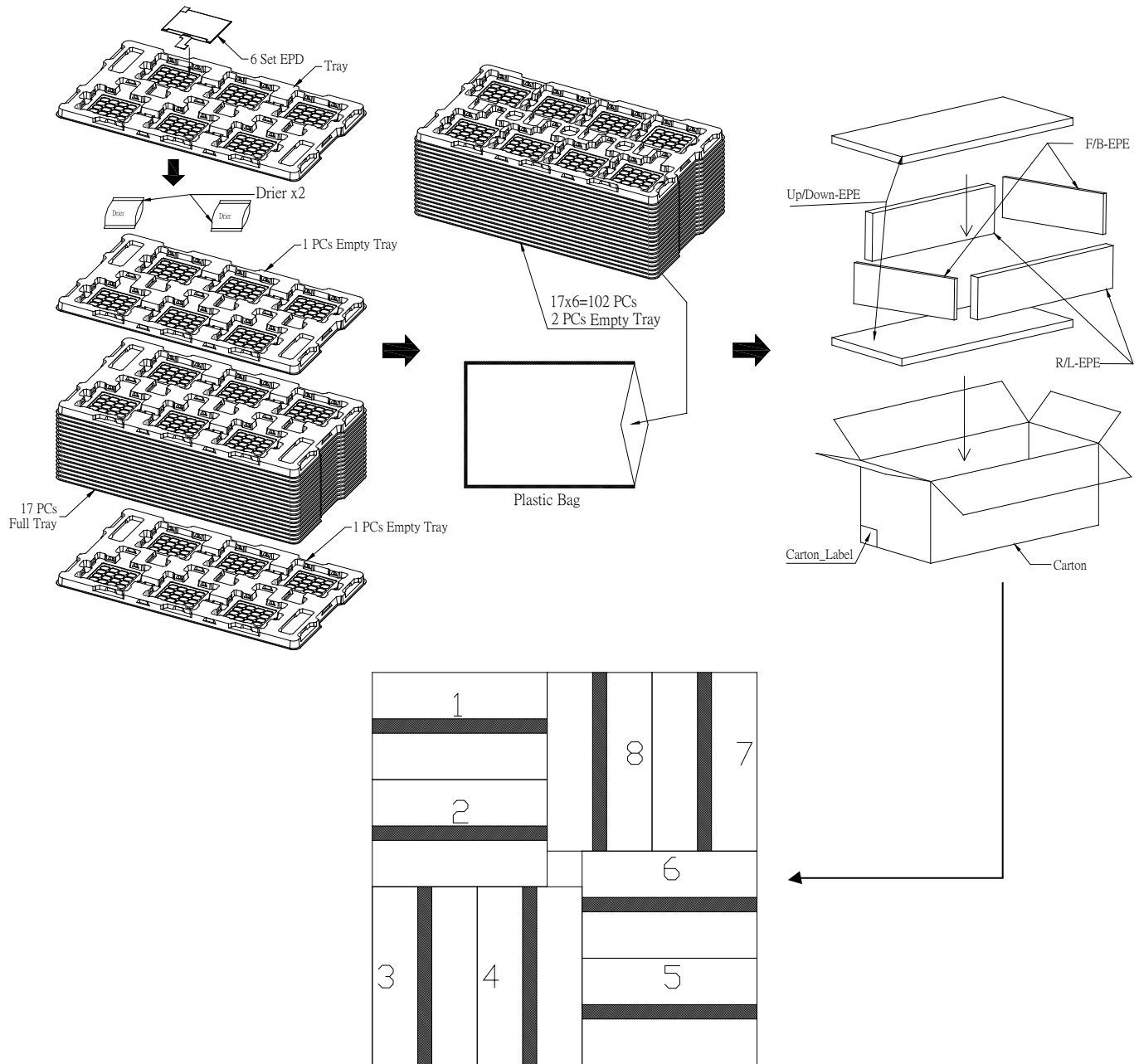
Figure 7-1 Packing Diagram
