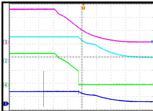
PG Shutdown through V_{IN}
