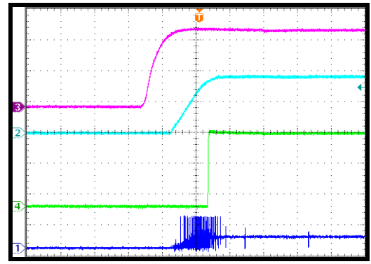
PG Start-Up through V_{IN}
