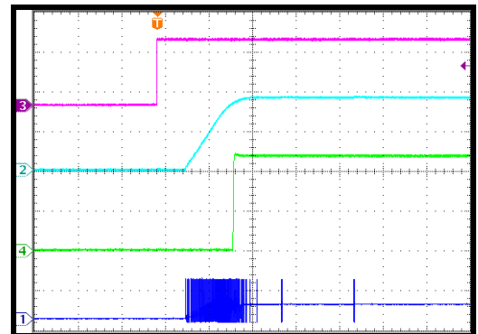
PG Start-Up through EN
