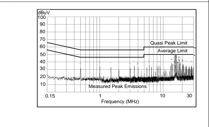
Figure 24. Conducted EMI Curve
