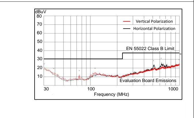
Figure 22. Radiated EMI Curve
