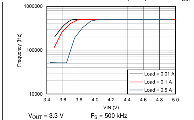
Figure 19. Switching Frequency vs V_{IN} in Dropout Operation
