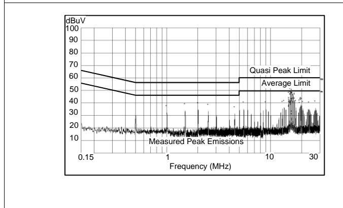
Figure 23. Conducted EMI Curve
