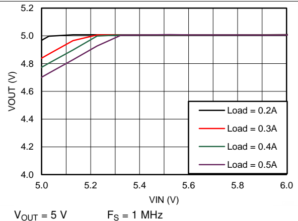
Figure 16. Dropout Curve
