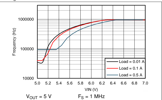
Figure 20. Switching Frequency vs V_{IN} in Dropout Operation
