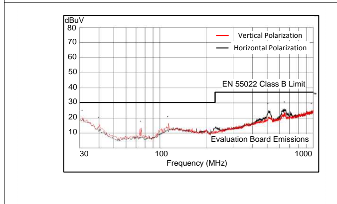
Figure 21. Radiated EMI Curve
