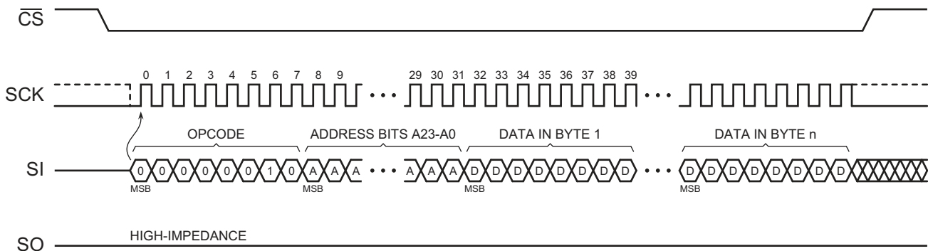
Figure 18. Page Program
