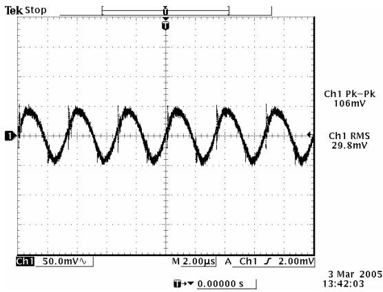
Ripple and noise at max load 12 Vdc/8.33 A output
