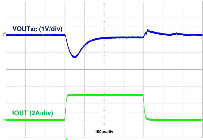
Figure 25. Load Transient, IOU T = 50mA to 3A to 50mA
