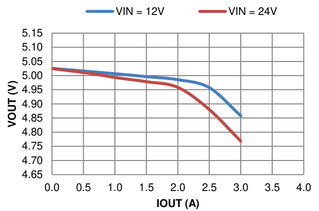
Figure 29. Load Regulation
