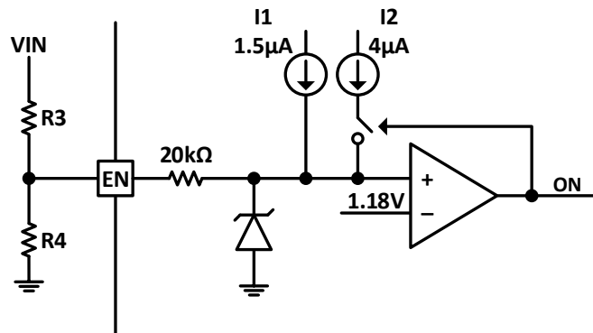
Figure 40. Adjusting UVLO
