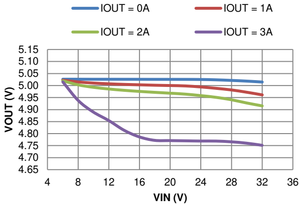
Figure 28. Line Regulation
