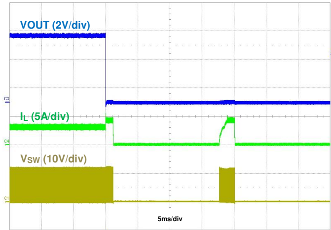
Figure 11. Output Short Protection, IOU = 3A
