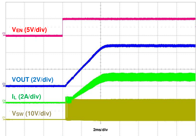
Figure 9. Startup using EN, IOU = 3A
