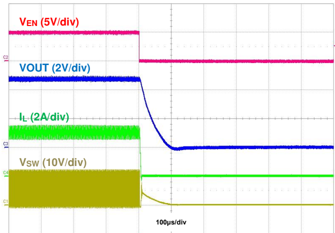
Figure 10. Shutdown using EN, IOU = 3A
