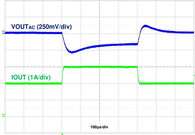
Figure 24. Load Transient, IOU T = 2A to 3A to 2A
