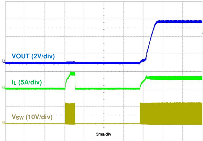
Figure 12. Output Short Recovery, IOU = 3A
