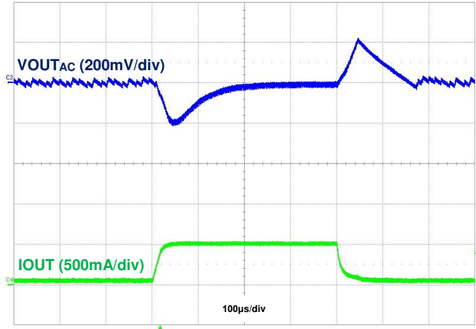
Figure 23. Load Transient, IOU T = 50mA to 500mA to 50mA
