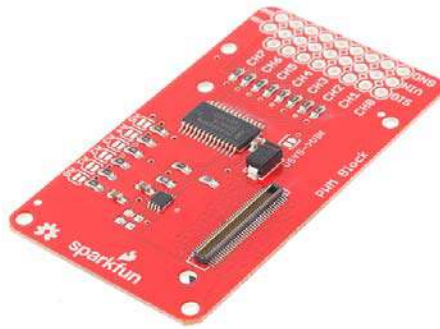
PWM Block
