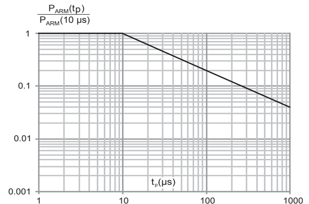
Figure 6. Normalized avalanche power derating versus pulse duration ( T_j = 125 ^{\circ}C )
