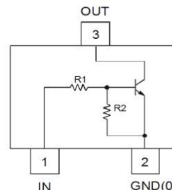
Device Schematic
