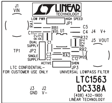
Silkscreen Top
