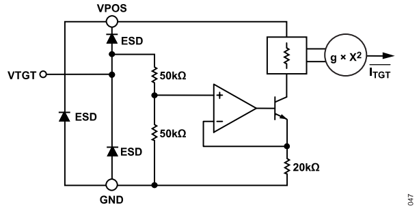
Figure 49. VTGT Interface
