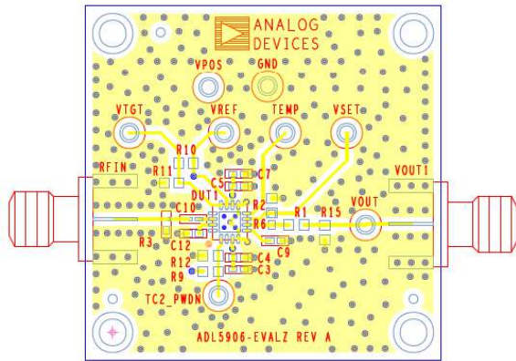
Figure 64. ADL5906 Evaluation Board Layout, Top Side
