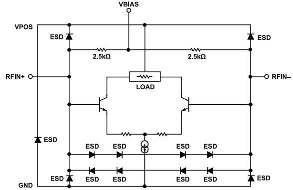
Figure 42. RF Inputs
