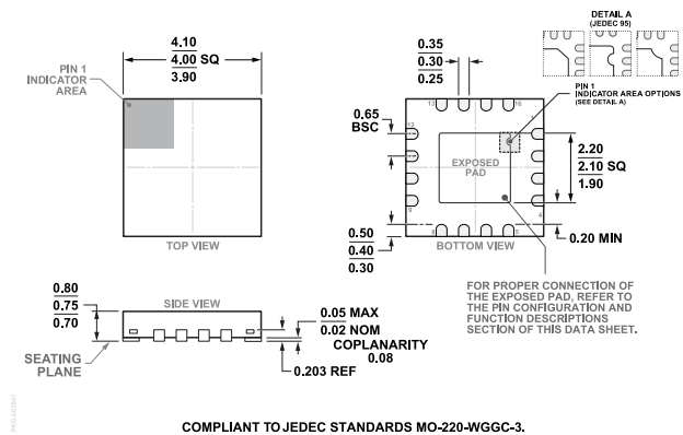
Figure 66. 16-Lead Lead Frame Chip Scale Package [LFCSP_WQ] 4 mm × 4 mm Body, Thin Quad (CP-16-59) Dimensions shown in millimeters
