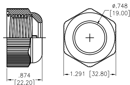
Ⓔ Sealing Nut
