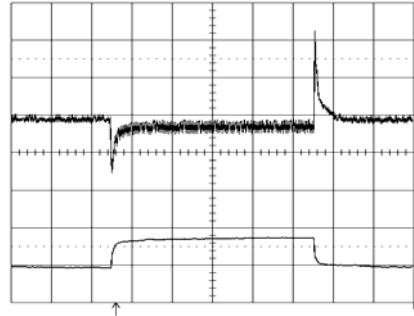
Output voltage response to load current step- change (15-30-15 A) at: T_{ref} = +25^{\circ}C , V_i = 5.0 V. Top trace: output voltage (100mV/div.). Bottom trace: load current (20 A/div.). Time scale: 0.1 ms/div..
