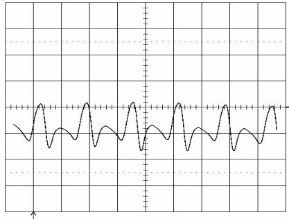
Output voltage ripple (20mV/div.) at: T_{ref} = +25^{\circ}C , I_O = 30 A resistive load, V_i = 5.0 V. Time scale: 2 \mu s/div. See the filter in the Output ripple and noise section (EMC Specification).
