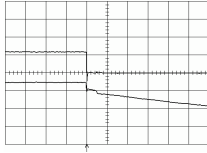
Shut-down enabled by disconnecting V_i at: T_{ref} = +25^{\circ}C , I_O = 30 A resistive load, V_i = 5.0 V. Top trace: output voltage (1.0 V/div.). Bottom trace: input voltage (2 V/div.). Time scale: 5.0 ms/div..
