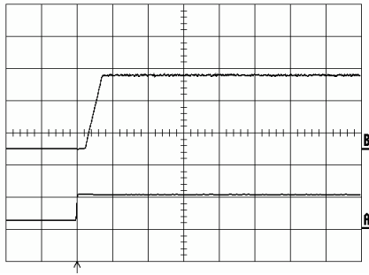
Start-up enabled by connecting V_i at: T_{ref} = +25^{\circ}C , I_O = 30 A resistive load, V_i = 5.0 V. Top trace: output voltage (0.5 V/div.). Bottom trace: input voltage (5 V/div.). Time scale: 10 ms/div..
