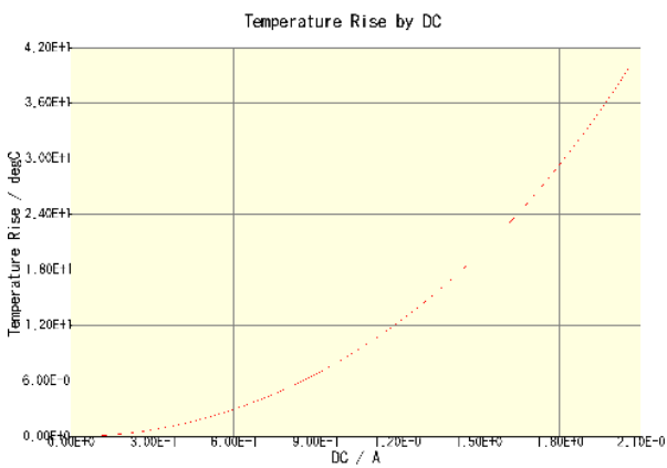
CLF12555T-470M-CA(Amb. Temp. = 20degc)
