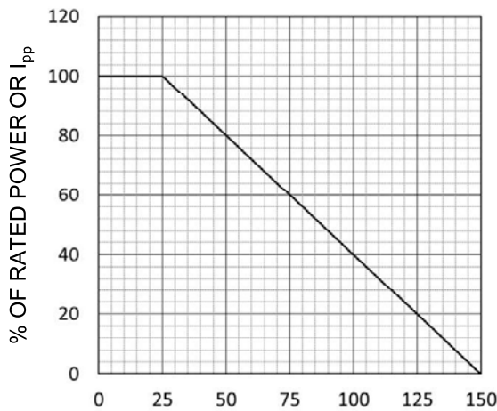
T_a (°C) POWER DERATING CURVE
