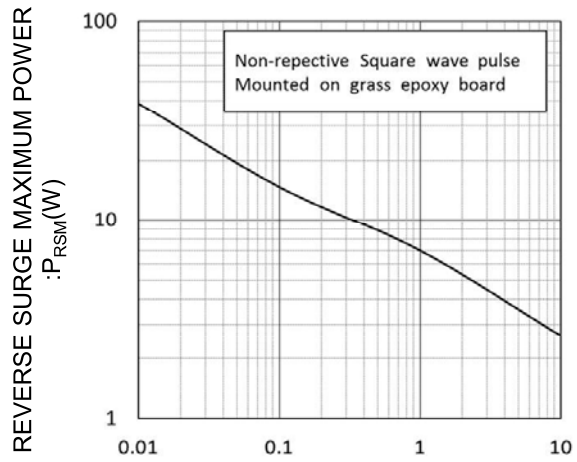
PULSE TIME: t (ms) P_{RSM} \cdot t CHARACTERISTICS
