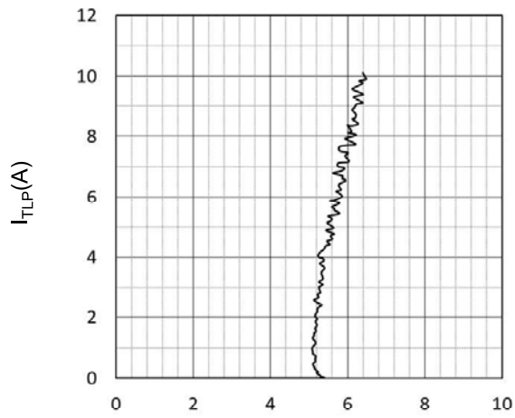
V_{TLP} (V) TRANSMISSION LINE PULSE
