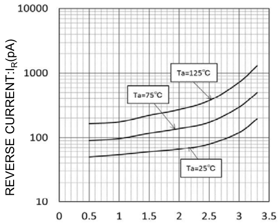
REVERSE VOLTAGE:VR(V) VR-IR CHARACTERISTICS
