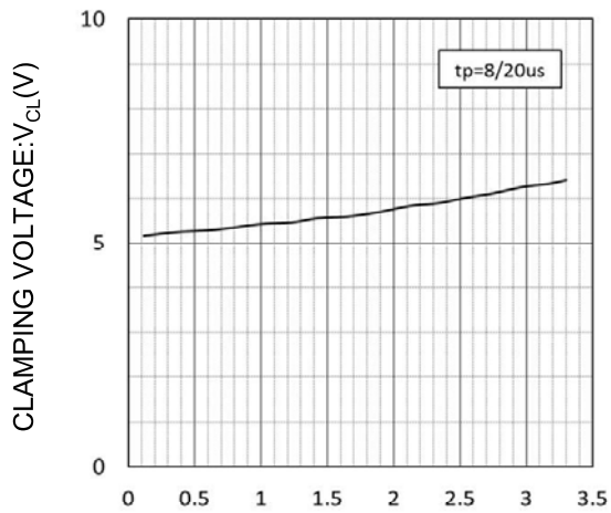
PEAK PULSE CURRENT: I_{pp} (A) CLAMPING VOLTAGE vs PEAK PULSE CURRENT
