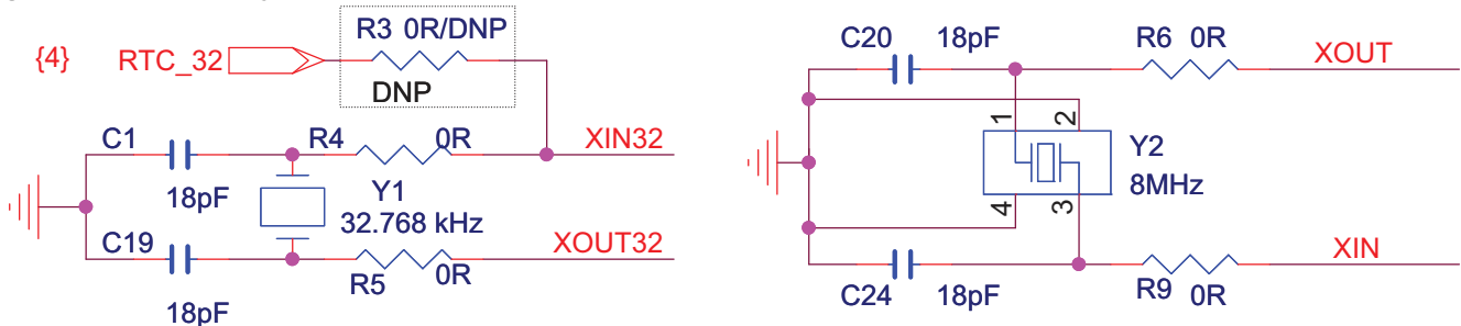
Figure 3-4. Clock System
