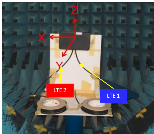
High High Band measured at 2550 MHz
