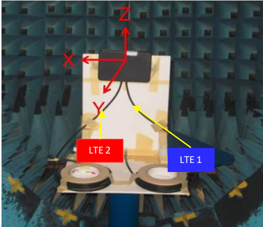
Low Band measured at 750 MHz
