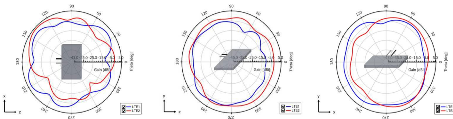
High High Band measured at 2550 MHz
