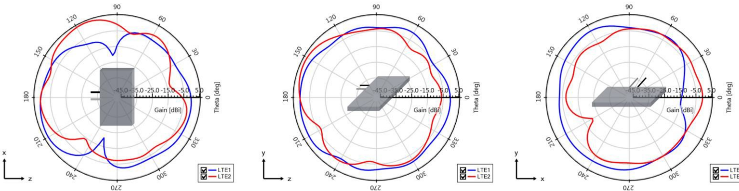
High Band measured at 1750 MHz
