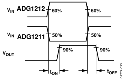
Figure 23. Switching Times
