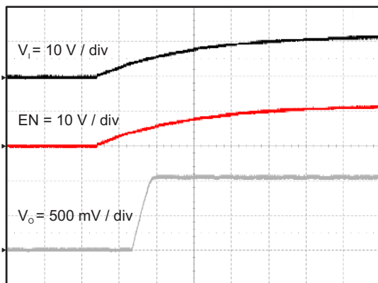
Figure 8-12. Tps562200 Start Up Relative to V 1
