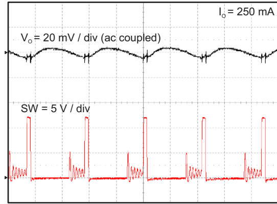
Figure 8-9. Tps562200 Output Voltage Ripple
