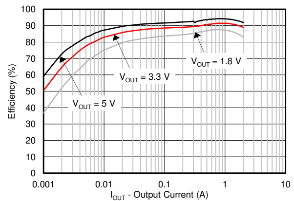
Tps562200 Efficiency
