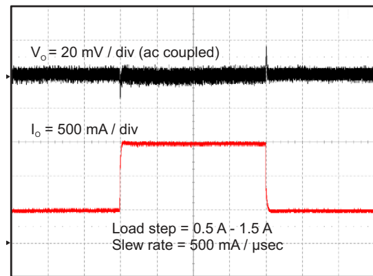
Figure 8-11. Tps562200 Transient Response
