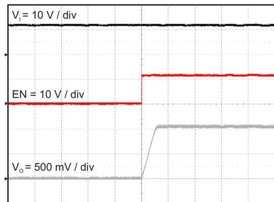
Figure 8-13. Tps562200 Start Up Relative to En
