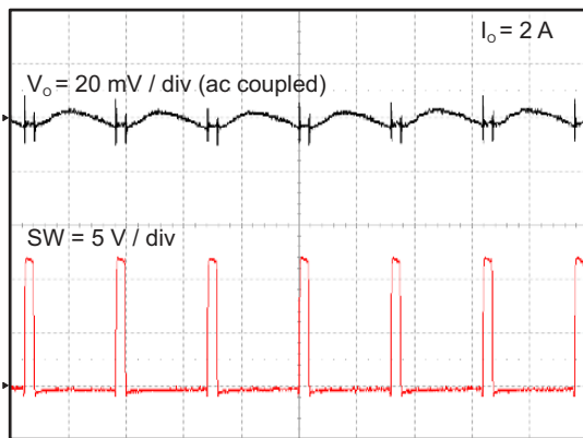
Figure 8-10. Tps562200 Output Voltage Ripple
