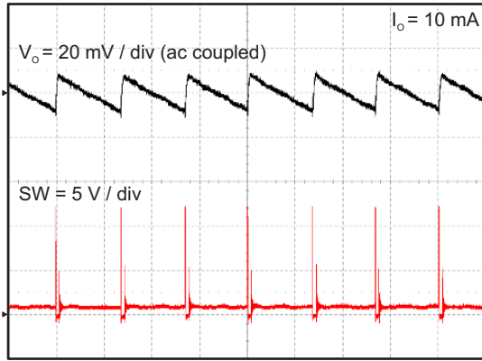
Figure 8-8. Tps562200 Output Voltage Ripple
