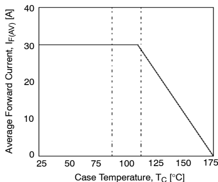
Figure 10. Forward Current Derating Curve
