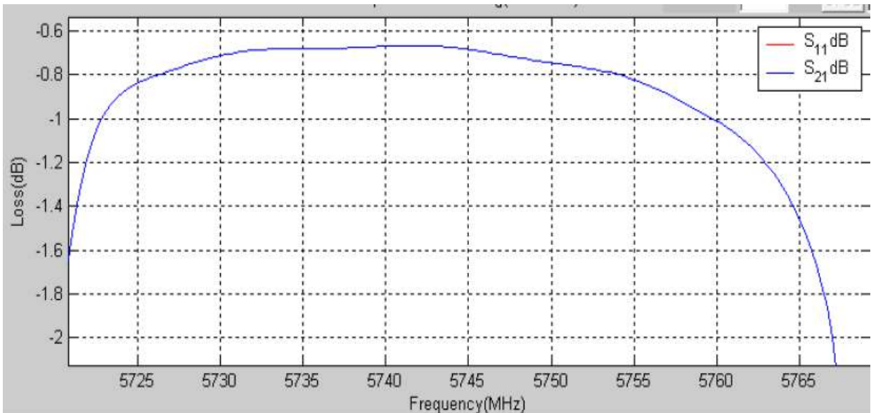
Figure2 Insertion loss
