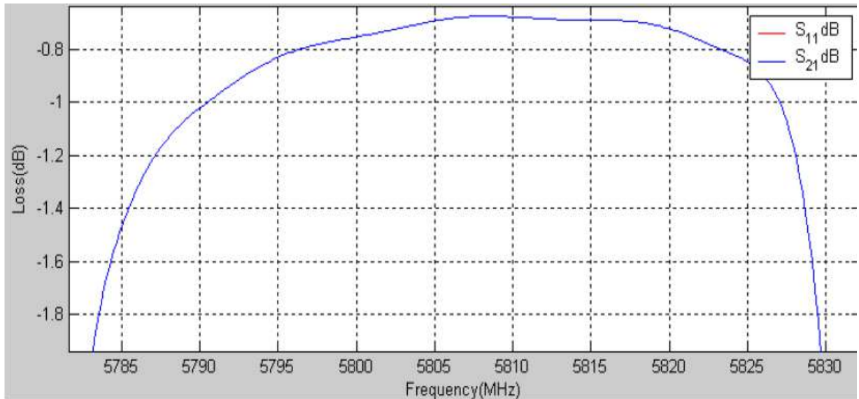
Figure2 Insertion loss
